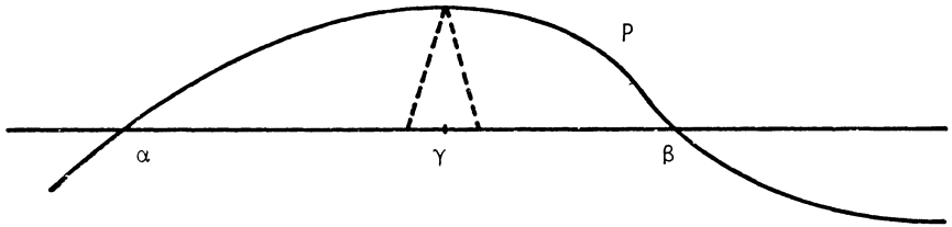
FIGURE 1 Minimum real root separation
